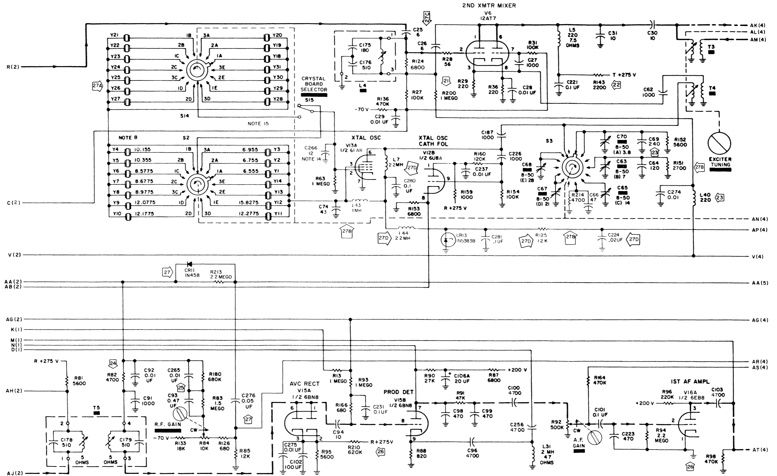
KWM-2 and KWM-2A Transceivers, Schematic Diagram Figure 7-1 (Sheet 3)
