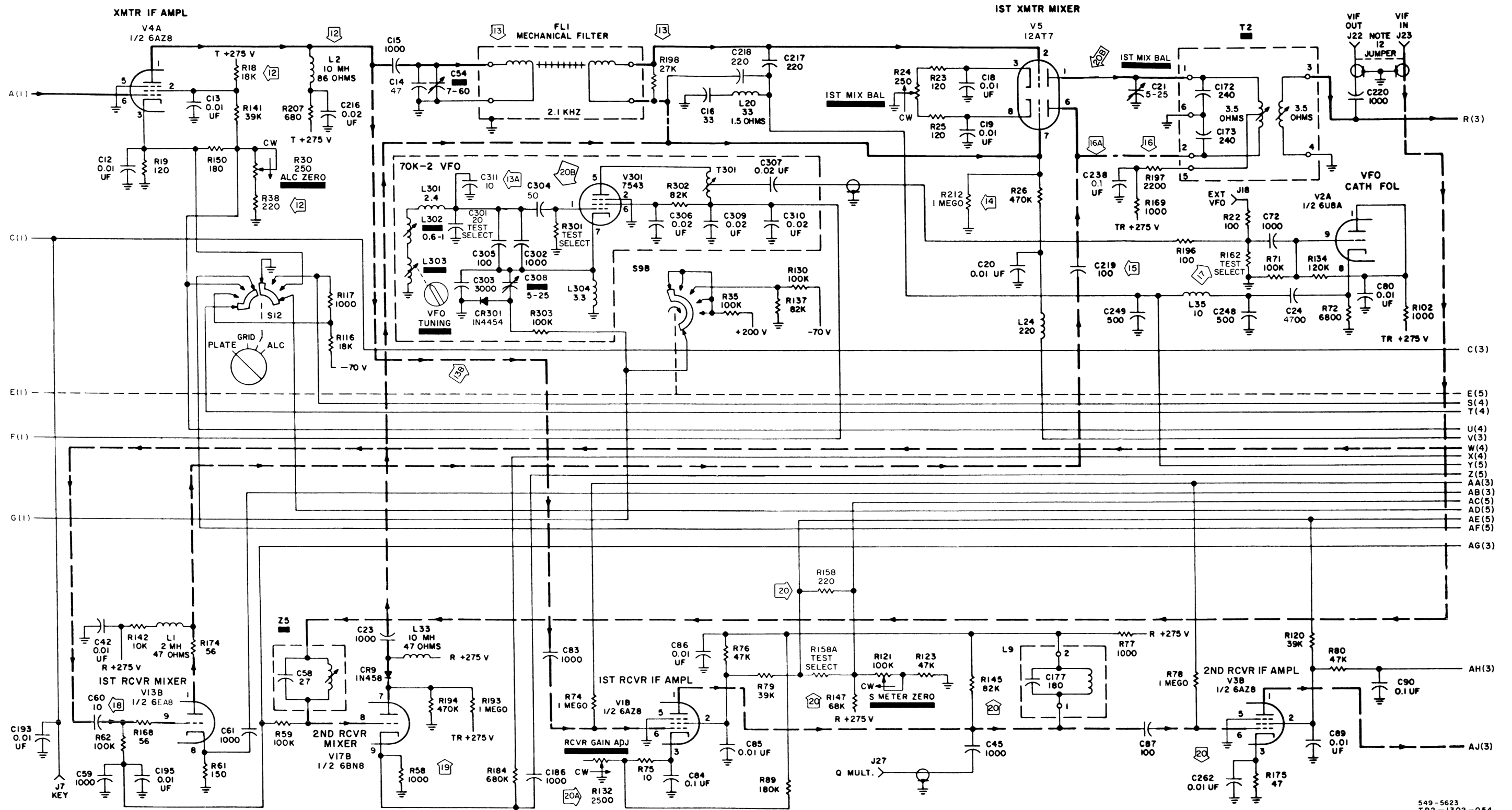
KWM-2 and KWM-2A Transceivers, Schematic Diagram Figure 7-1 (Sheet 2)
